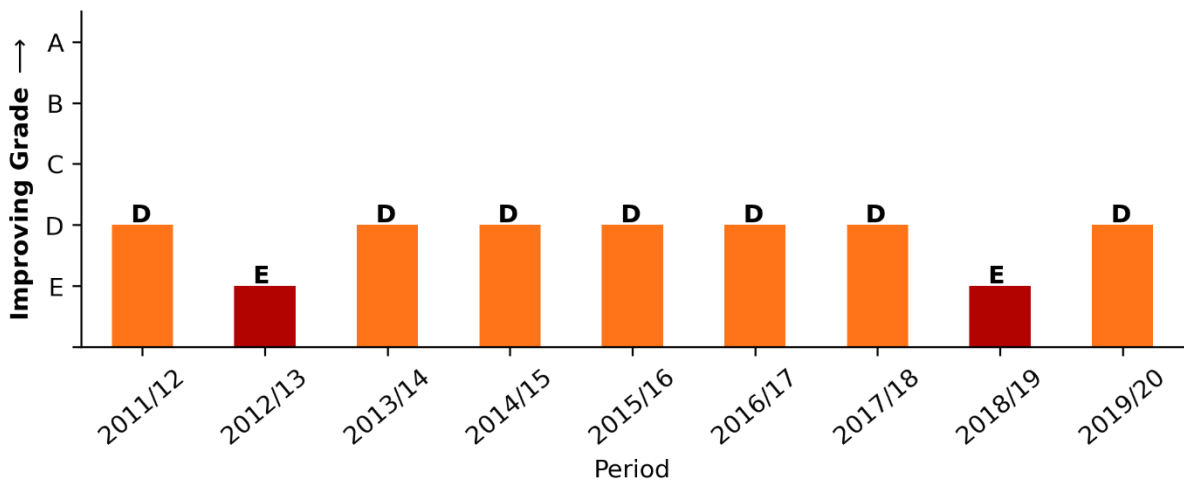
A.12: Grading of chlorophyll-a within Manly Lagoon as compared to other NSW estuaries
