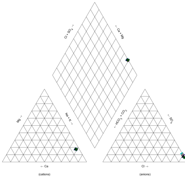
A.7: Piper diagram for surface water in Manly Lagoon
