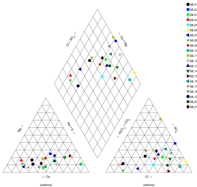
A.8: Piper plot for Manly Lagoon groundwater (dry conditions)
