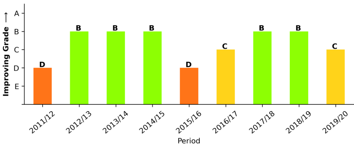
A.11: Grading of turbidity within Manly Lagoon as compared to other NSW estuaries
