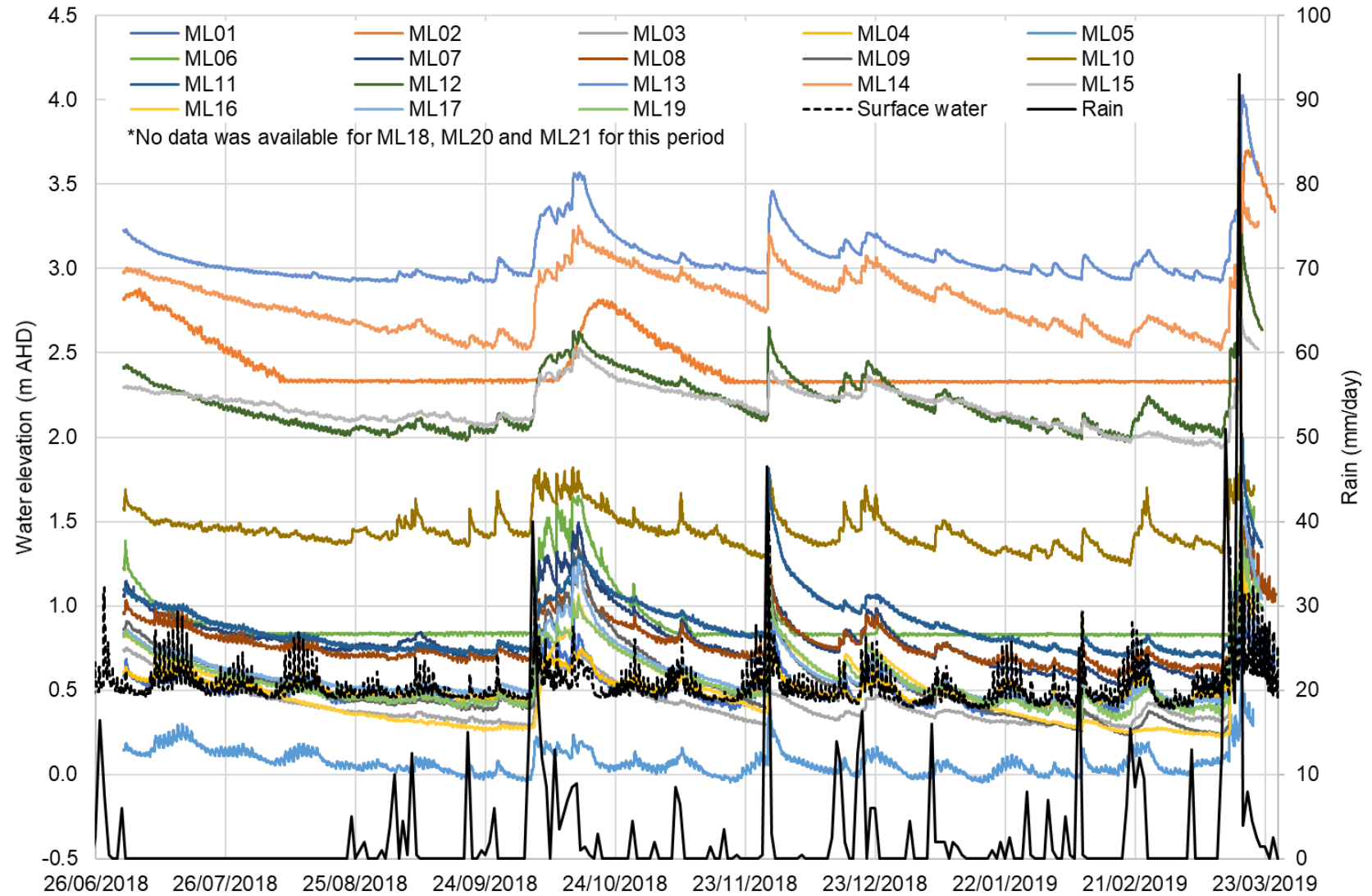
A.9: Groundwater levels as recured by data loggers for each borehole (2018-2019)
