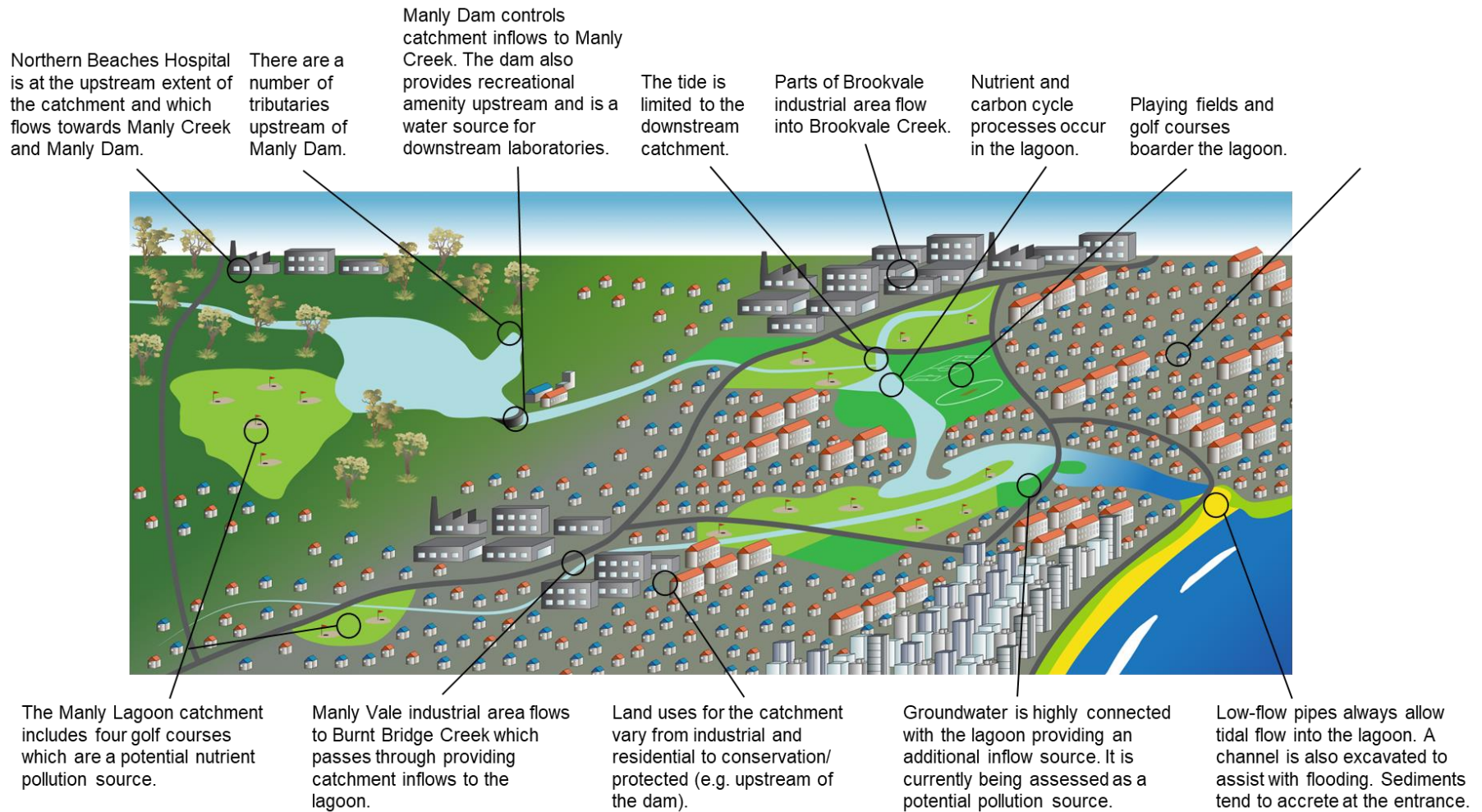
Figure ES.1: Conceptual environmental processes across the Manly Lagoon catchment
