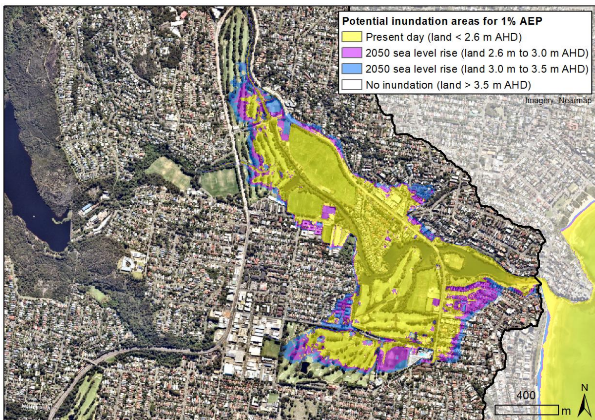
Figure 4.5: Manly Lagoon coastal inundation zones (including wave and wind setup) (Mariani et al., 2012)
