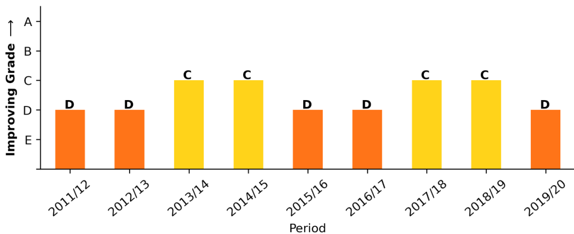
A.13: Overall grading for Manly Lagoon as compared to other NSW estuaries
