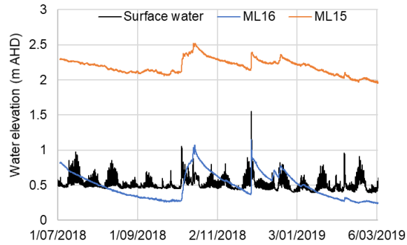
A.10: Comparison of groundwater and surface water levels (2018 to 2019)
