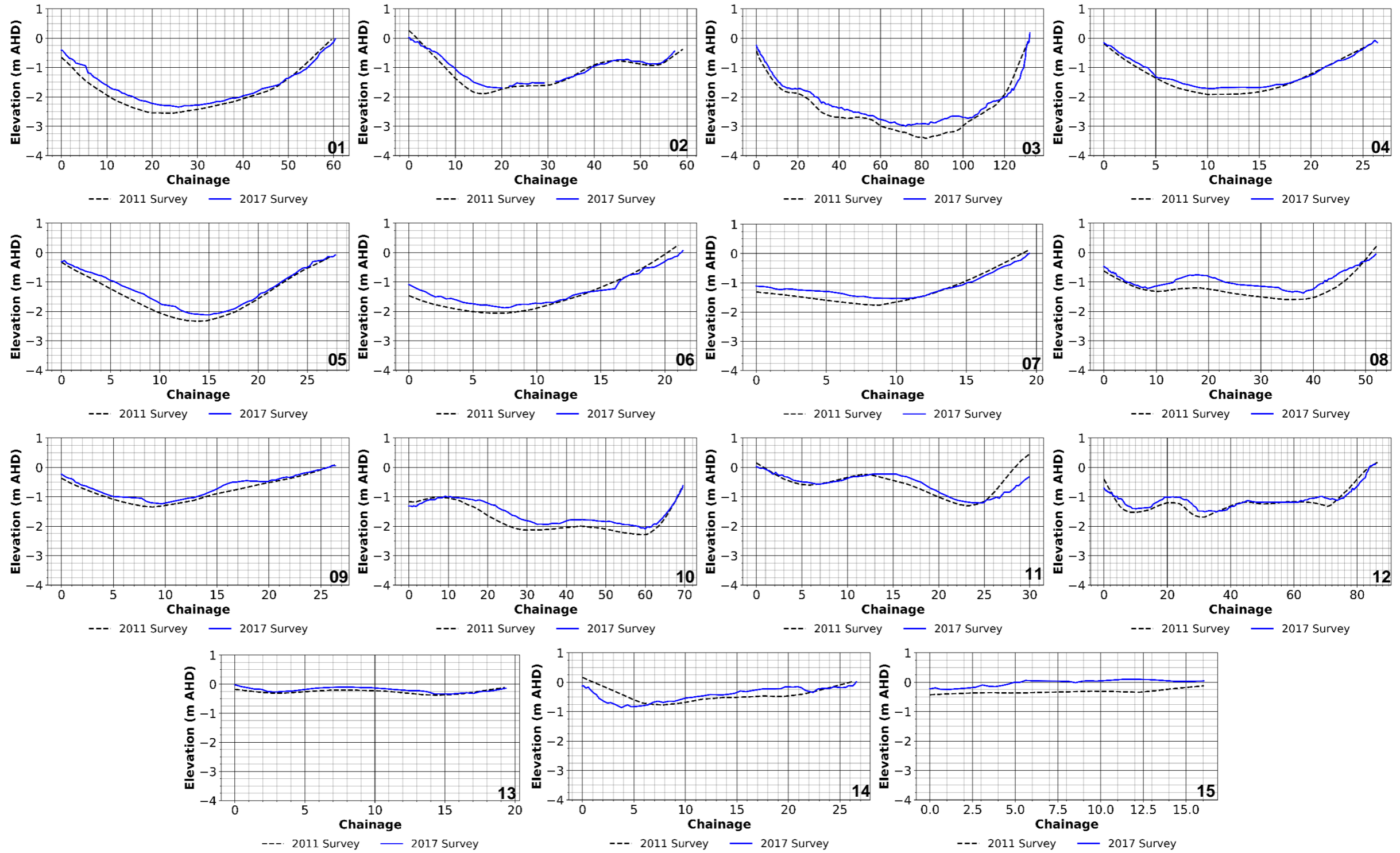
A.15: Comparison of bathymetry measurements between 2011 and 2017 (see locations in Figure A.14)
