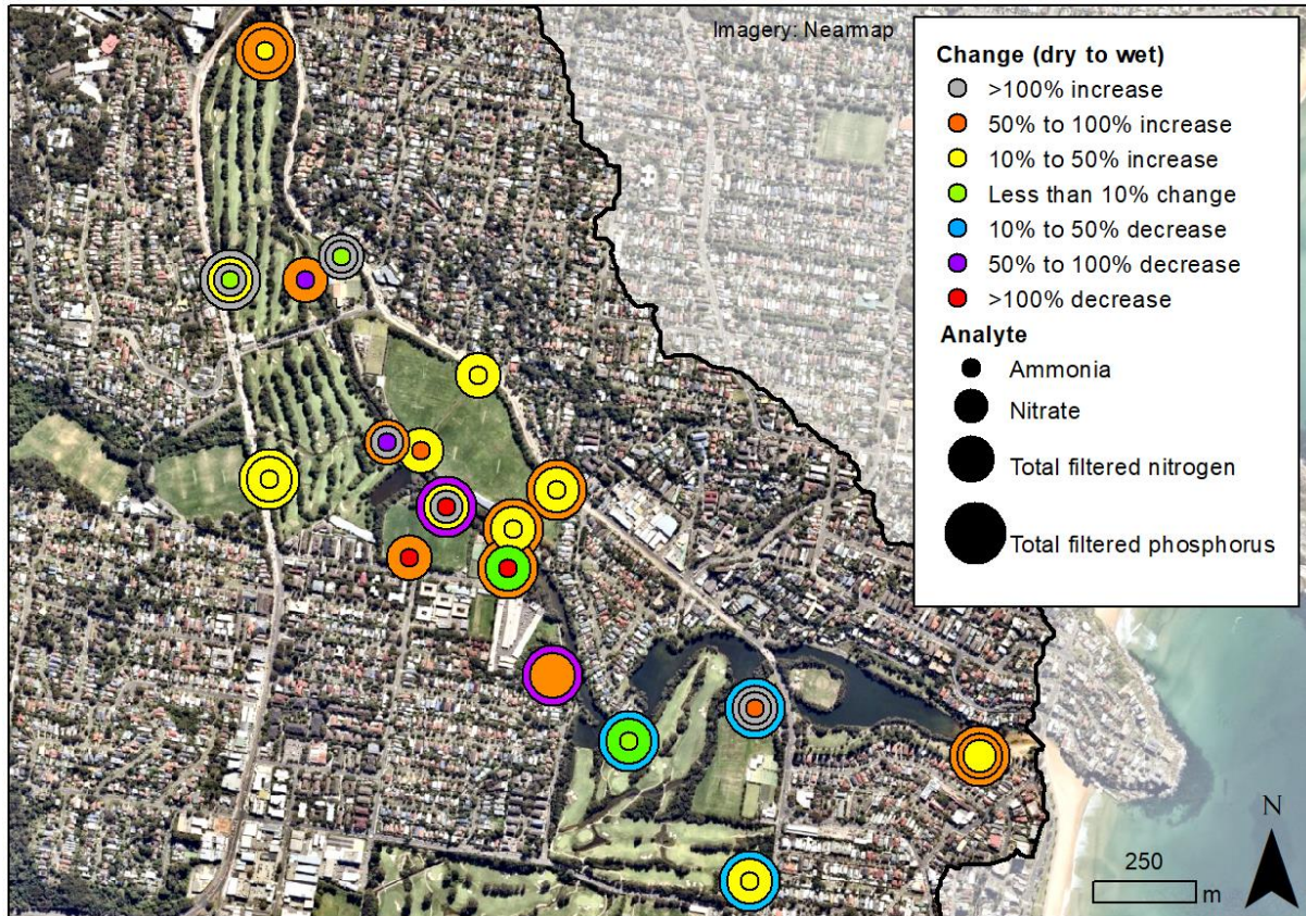
A.4: Comparison of nutrients sampled in wet versus dry conditions at Manly Lagoon
